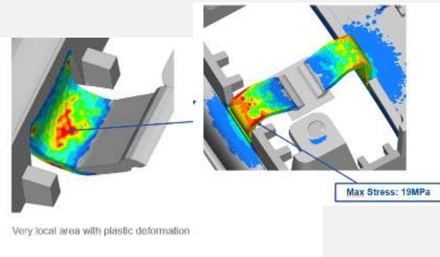
CAE Analysis
